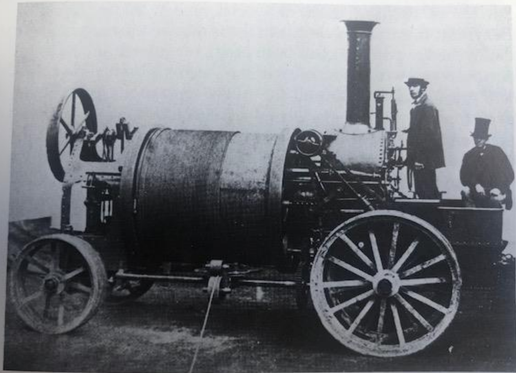
Benjamin Bomford's first ploughing engine, the Savory, built at Gloucester.
