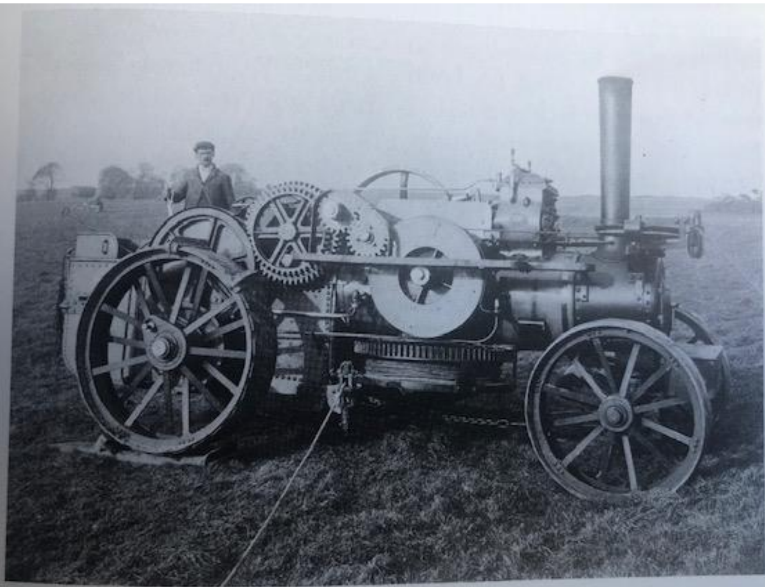
Most of the subsequent engines were Fowlers. This one is a double drum type.
